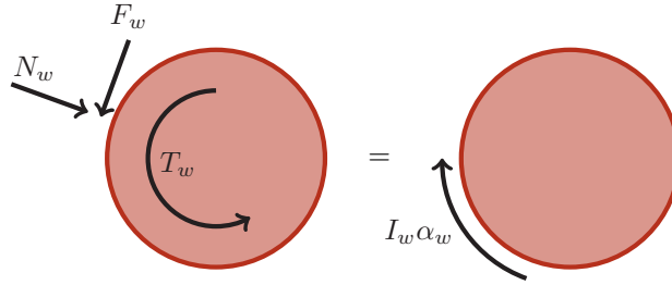
Figure 8: Free-Body and Kinetic Diagrams for Wheel
